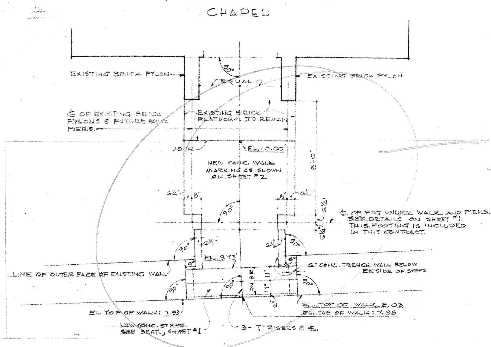
PLAN OF WORK IN THIS CONTRACT. SCALE: 1/4" = 1'-0"
