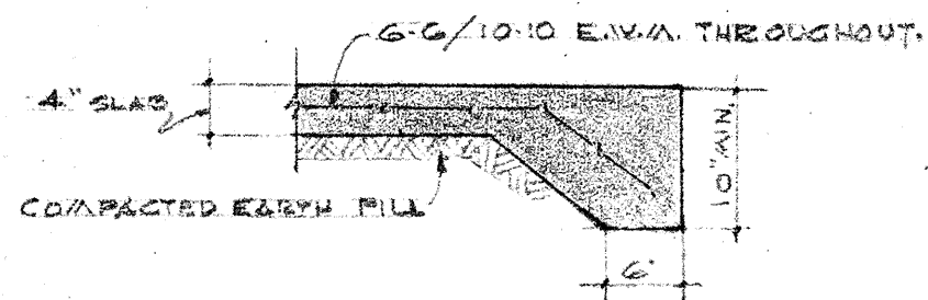
SECT. THRU NORTH & SOUTH EDGES OF WALK. SCALE: 3/4" = 1'-0"
